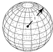
Source: Wolfram Research unit sphere in 4D
