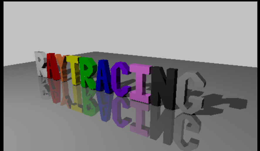
Raytracing
