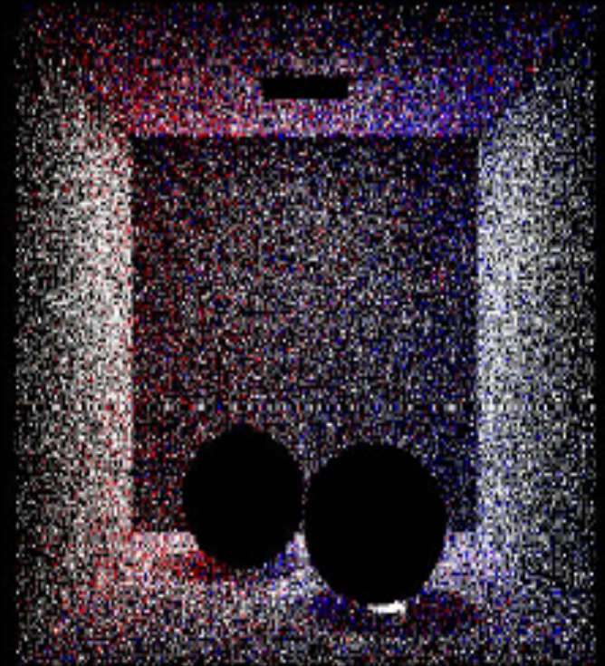
Photon Map
