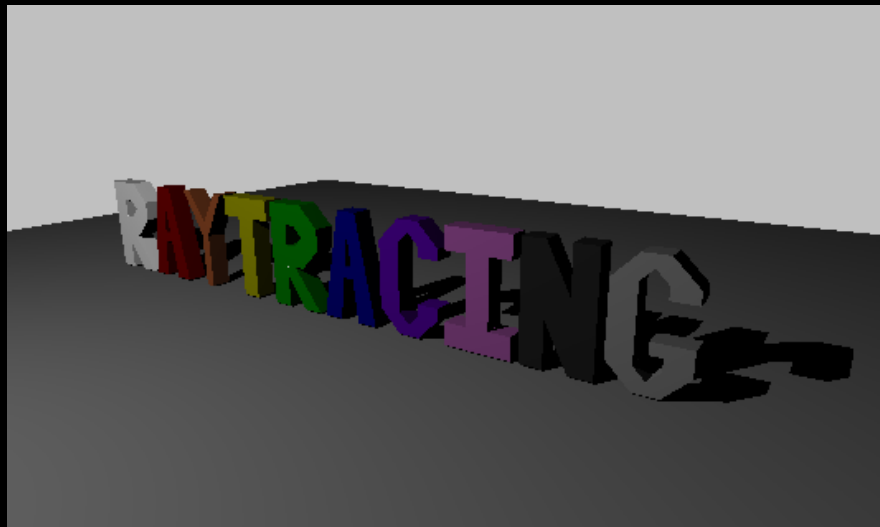
Raycasting
